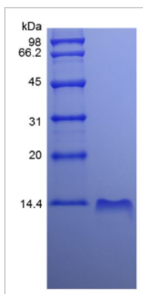
SDS-PAGE (Cat.No.: CXCL10-08H )
